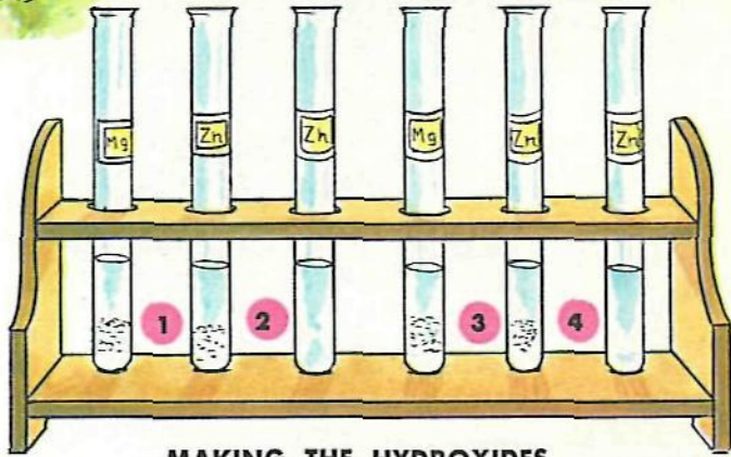
MAKING THE HYDROXIDES
