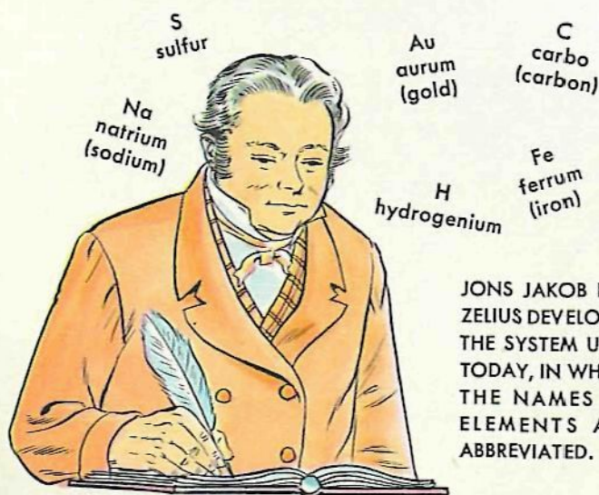
JOHN DALTON SUGGESTED MARKED CIRCLES TO INDICATE DIFFERENT ELEMENTS.
