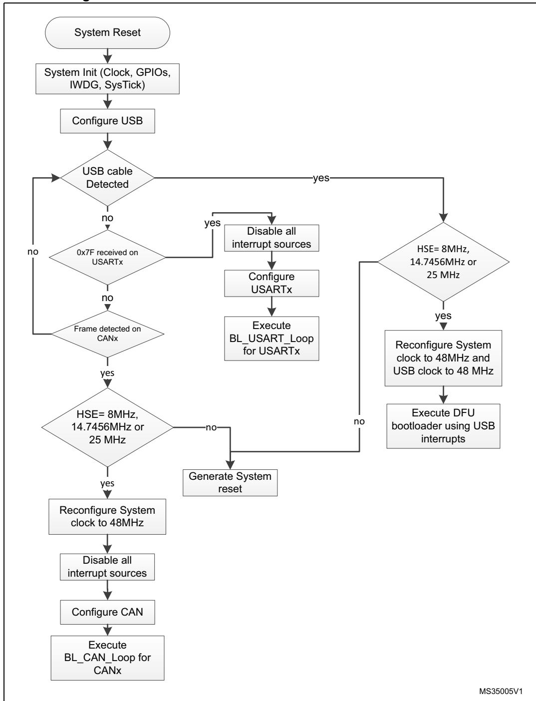
Figure 17. Bootloader selection for STM32F105xx/107xx devices
