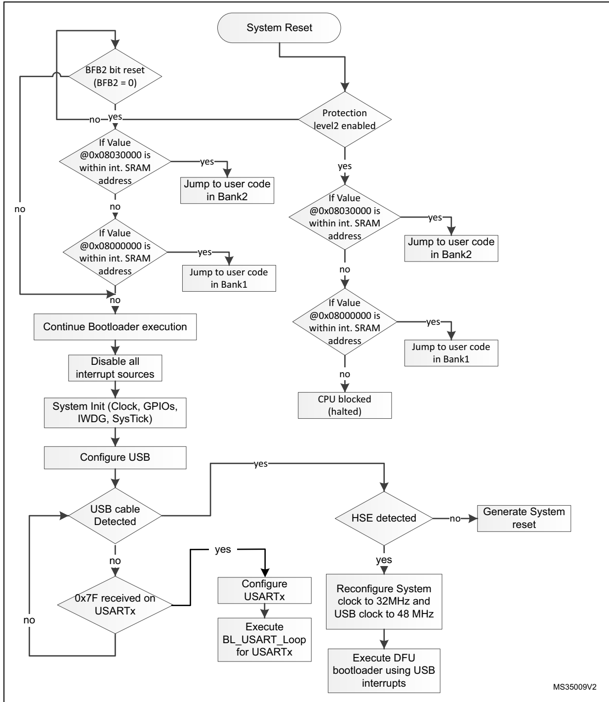
Figure 70. Bootloader selection for STM32L1xxxD devices
