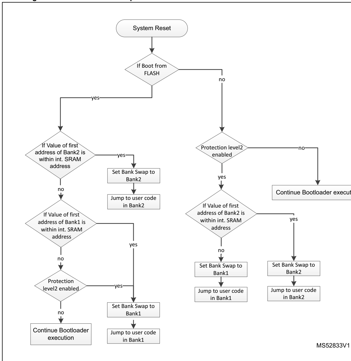
Figure 56. Dual bank boot implementation for STM32G47xxx/48xxx bootloader V13.x
