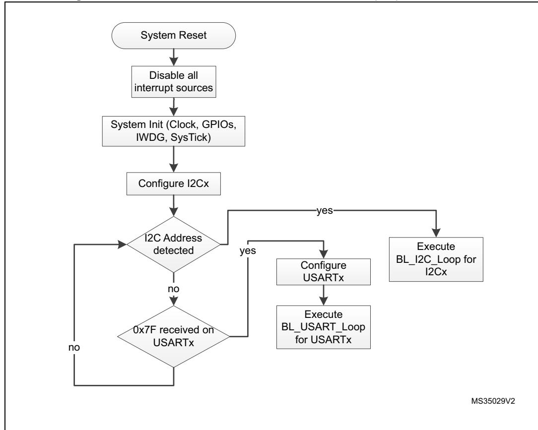
Figure 24. Bootloader selection for STM32F303x4(6/8)/334xx/328xx
