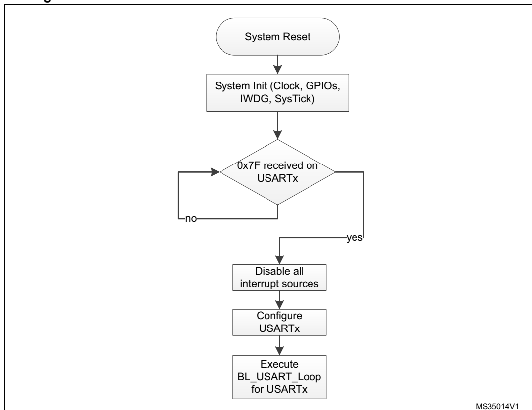
Figure 10. Bootloader selection for STM32F05xxx and STM32F030x8 devices
