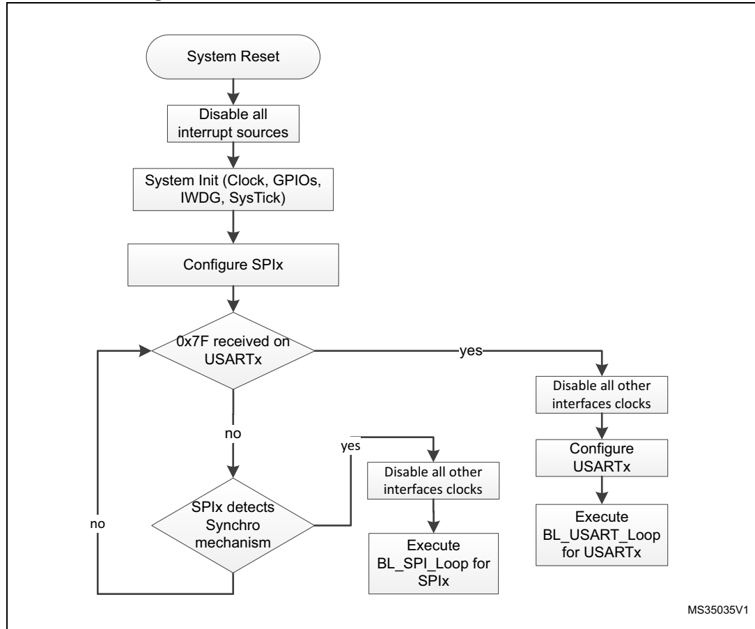
Figure 62. Bootloader selection for STM32L05xxx/06xxx
