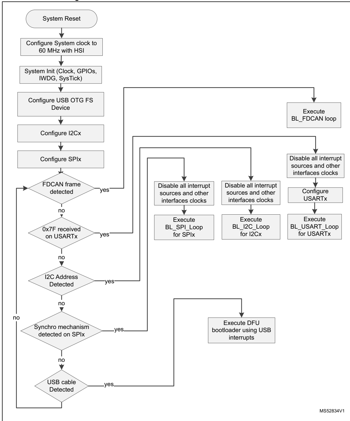
Figure 88. Bootloader V9.x selection for STM32L552xx/562xx
