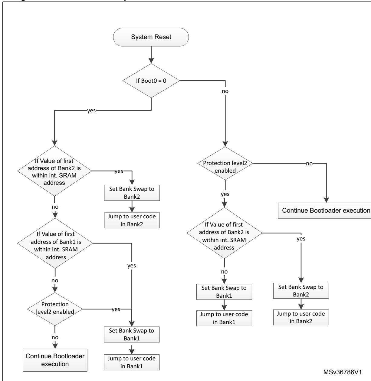
Figure 86. Dual bank boot implementation for STM32L4Rxxx/STM32L4Sxxx bootloader V9.x
