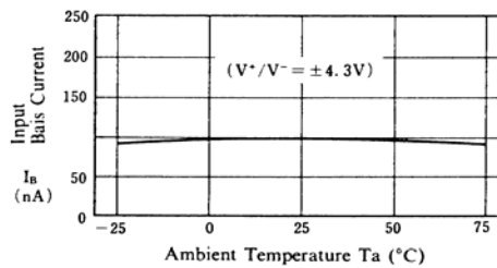
Input Bias Current vs. Temperature
