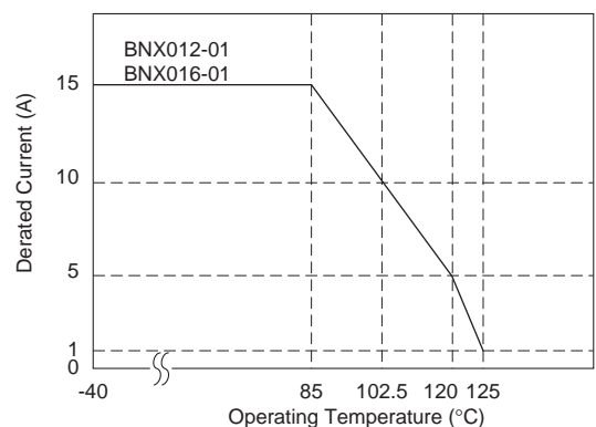
Derating
