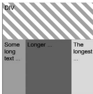
grid-auto-flow: row
